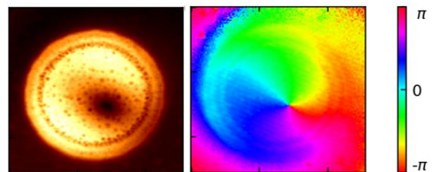
Figure 2 Near-field distribution of the amplitude (left) and phase (right) of the dipolar plasmonic resonance of a gold disk (diameter 1 \mu\text{m} ) upon light excitation with circular polarization
